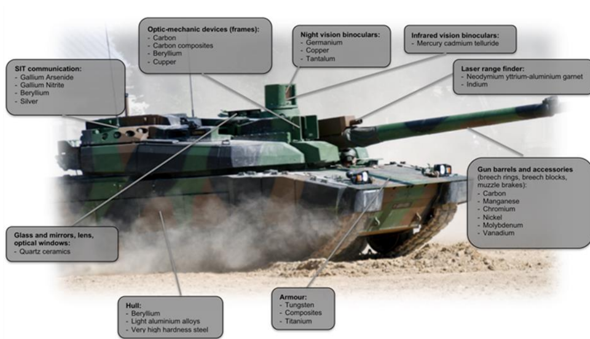
Figure 3.5: Components and raw materials used in a main battle tank (e.g. Leclerc), but also representative of infantry-fighting and armoured-fighting vehicles (source: CEIS)
